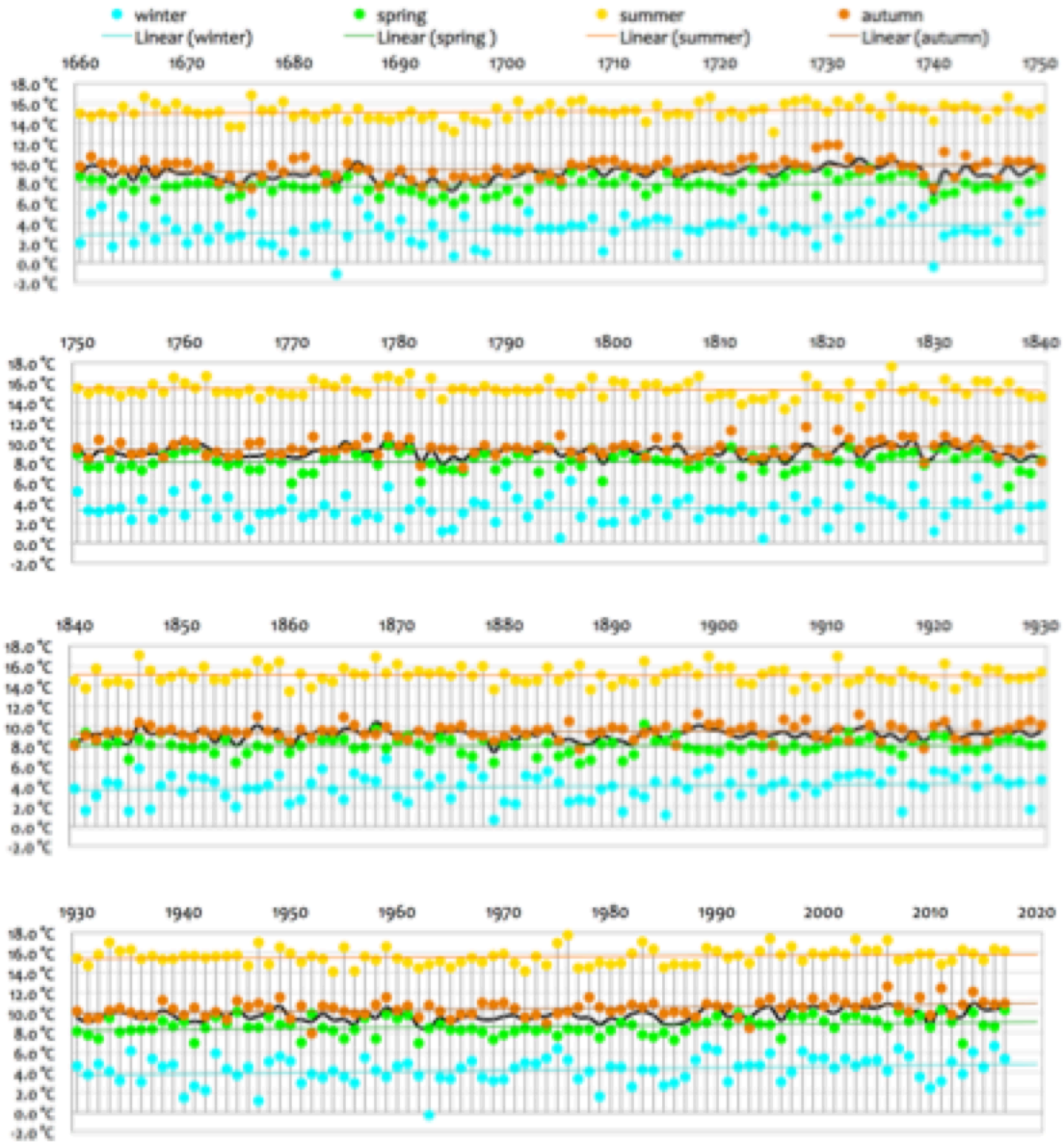
UK Met Office CET seasonal temperatures and trends: 1660 - 1750 - 1840 - 1930 - 2020
